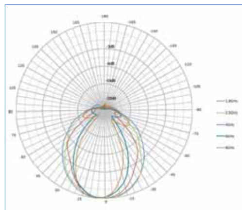
Vertical Pattern HyperLOG 3080 X
