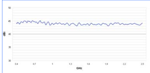
Gain diagram HyperLOG 4025X
