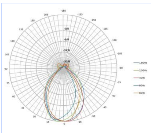
Horizontal Pattern HyperLOG 6080 X
