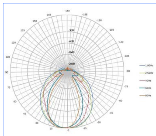
Vertical Pattern HyperLOG 6080 X
